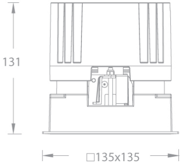
Line Drawing
